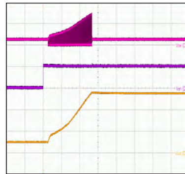
Start Up into Openload
