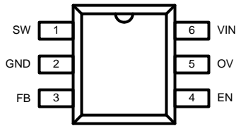
Top View: TSOT23-6
